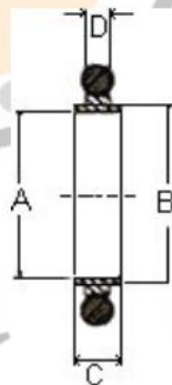
KF 304 Centering Ring, NBR O'ring
