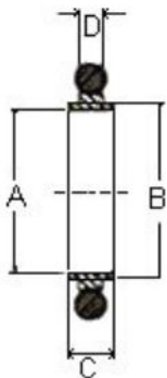
KF Aluminum Centering Ring, NBR O'ring
